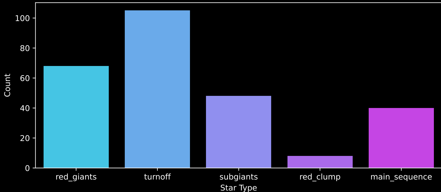
GALAH DR4 Field: [9273] Count plot of Star Type
