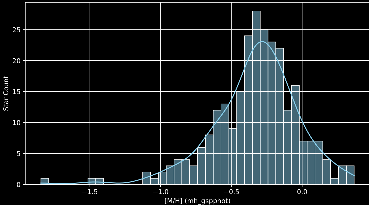
GALAH DR4 Field: [9273] [M/H] (mh_gspphot) (n= 267)
