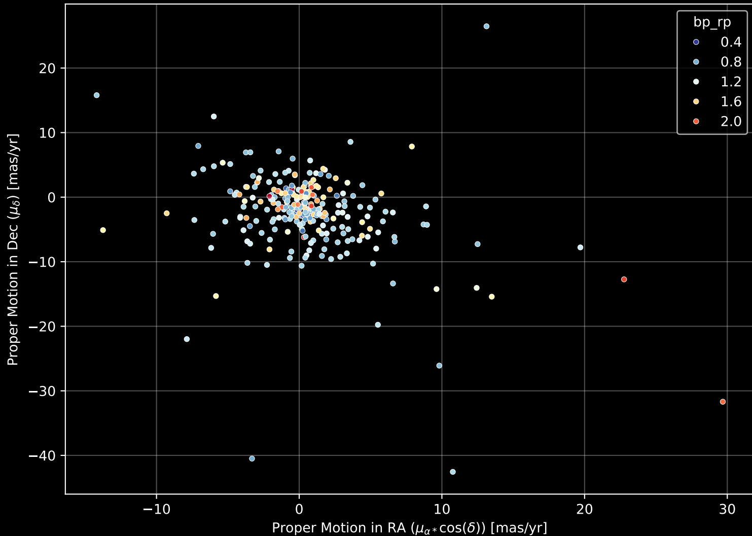
GALAH DR4 Field: [9273] Proper Motion Diagram (n= 269)
