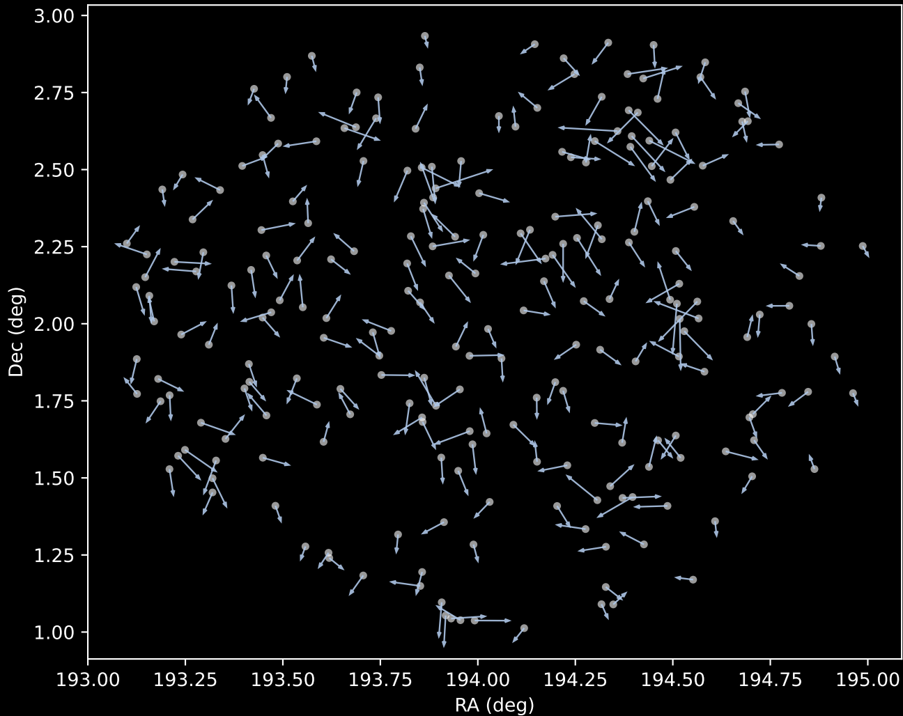
GALAH DR4 Cluster 1 Proper Motion Vectors (n=232)
