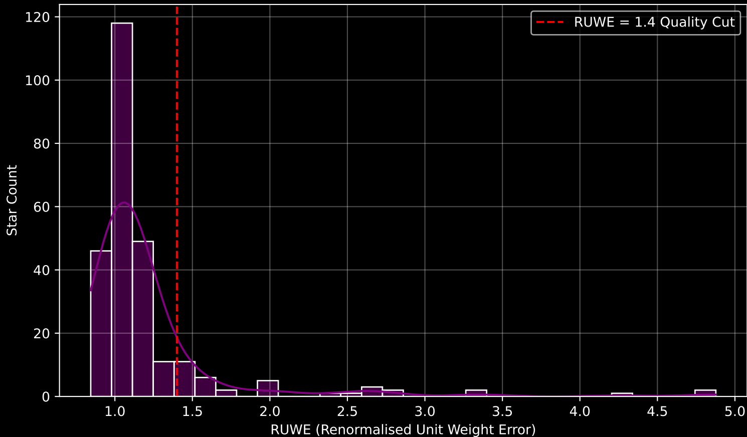
GALAH DR4 Field [9273] RUWE Distribution (n= 260)
